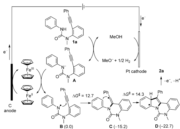
Scheme 5. Mechanistic proposal and computational studies. The values are DFT-derived energetics for the cyclization of the radical intermediate B . The energies ( \text{kcal mol}^{-1} ), shown within parentheses, are those relative to B and were calculated at the level of B3LYP/6-31G*.
