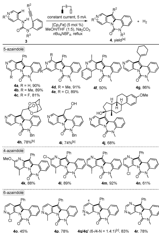
Scheme 3. Scope of azaindole synthesis. Reaction conditions were the same as those of Scheme 2. [a] Yield of isolated product. [b] The reaction time was 8 h (5 F). [c] Two separable isomers were obtained.
